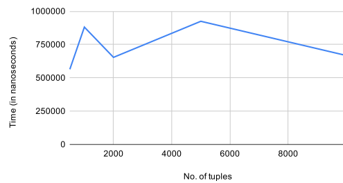
Join - HashMap (c)
