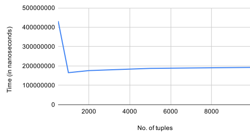
Join - NoIndex (a)
