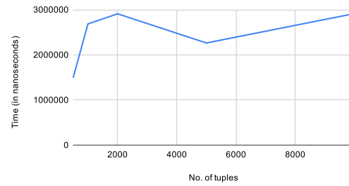
Join - TreeMap (b)
