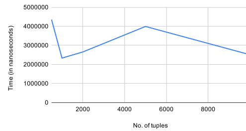
Select - NoIndex (a)
