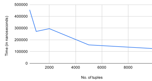
Select - HashMap (c)
